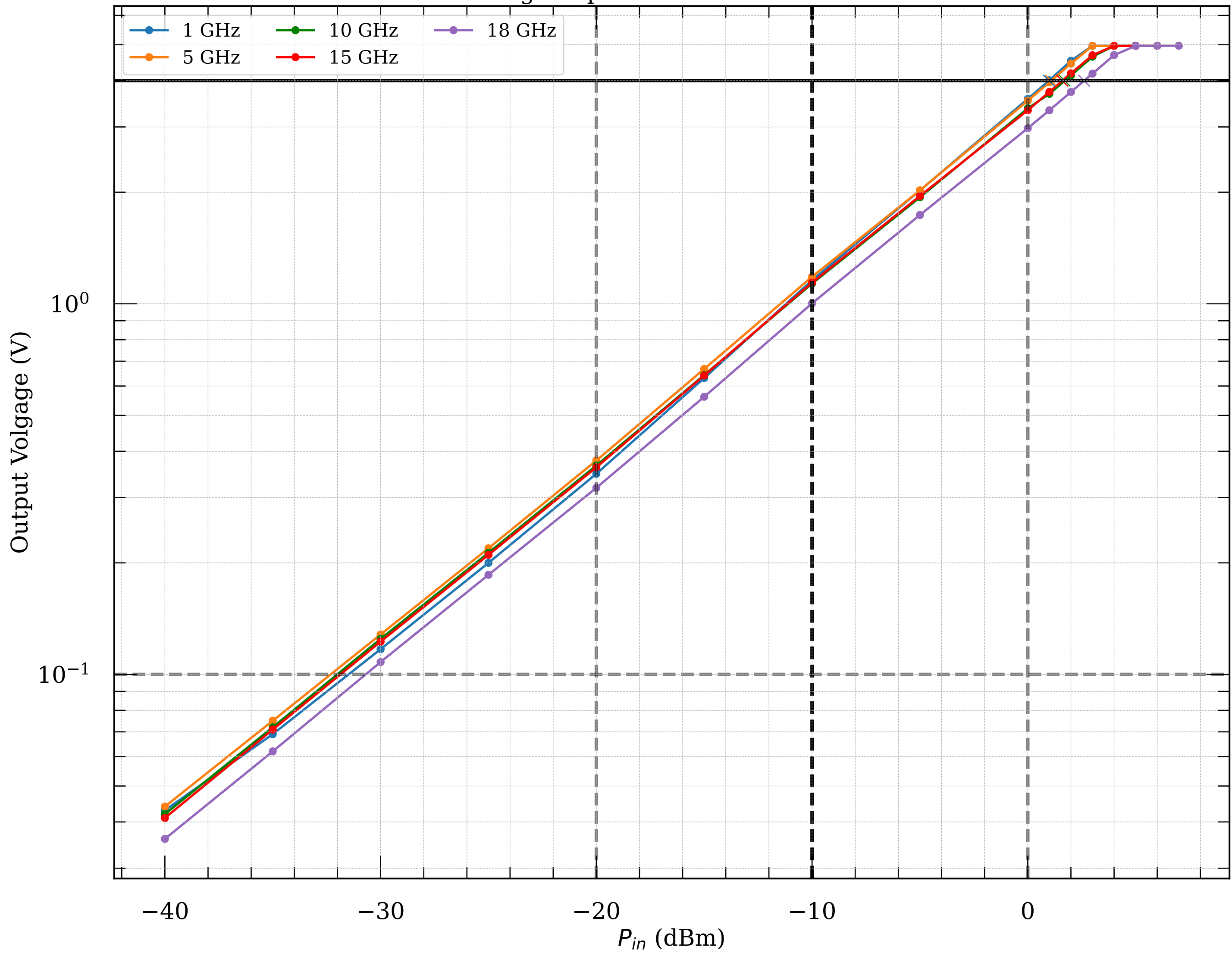
Measured voltage-to-power curve of detector module089
